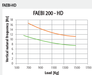
FAEBI® 200-HD
