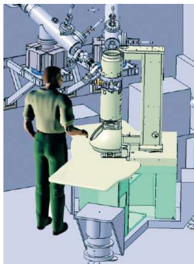
Platform for integration in double/clean room floors with additional mass for the reduction of vibration peaks
