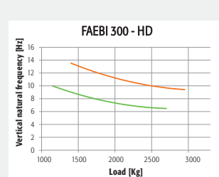
FAEBI® 300-HD
