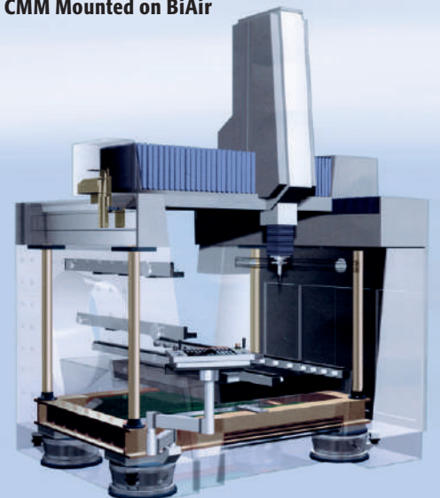
CMM Mounted on BiAir
