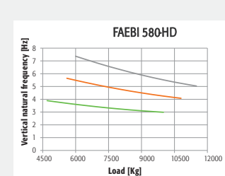
FAEBI® 580-HD
