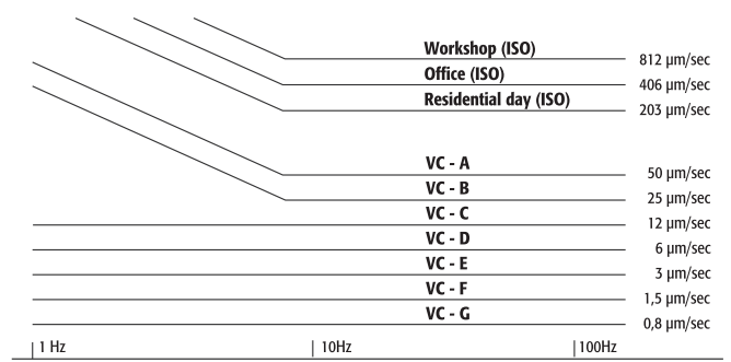
Chart 2: Vibration Criteria VC
